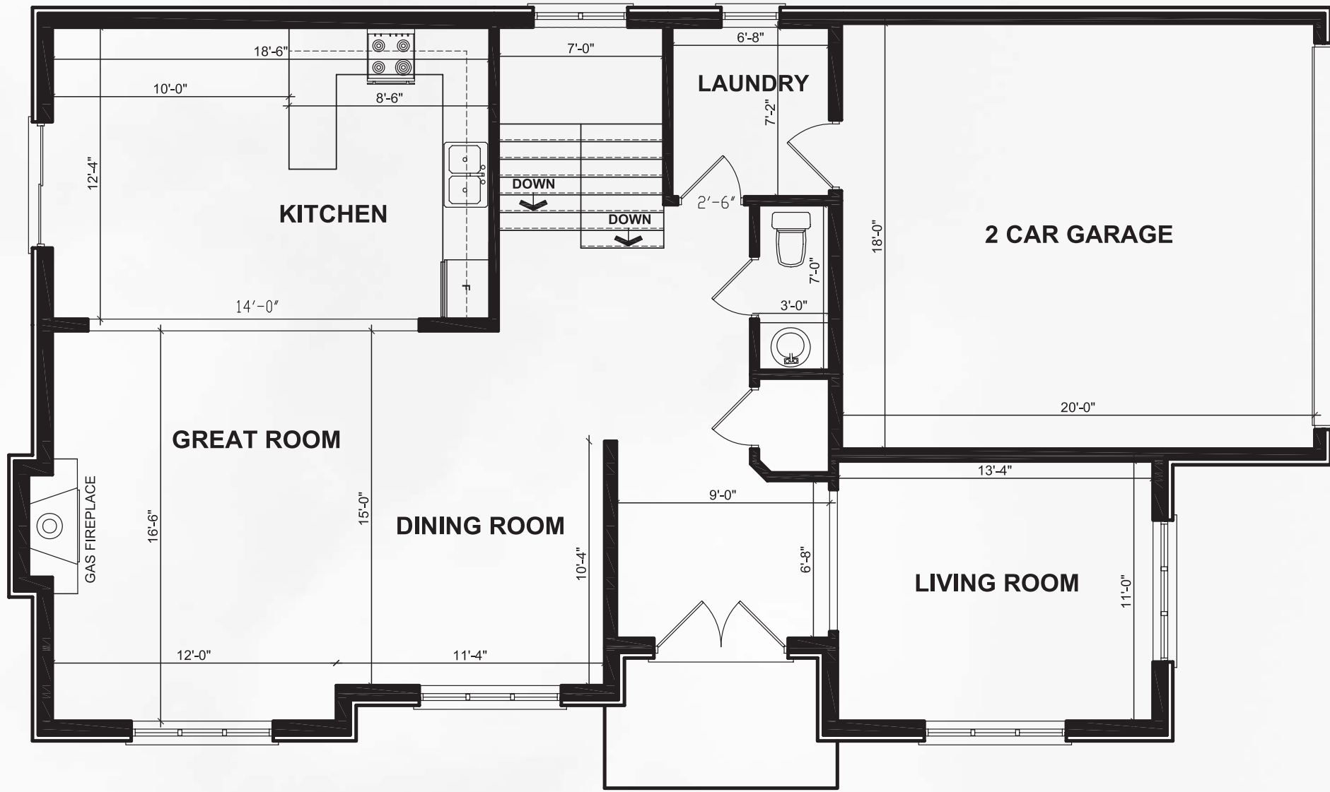
MAIN FLOOR 1186 sq.ft.
