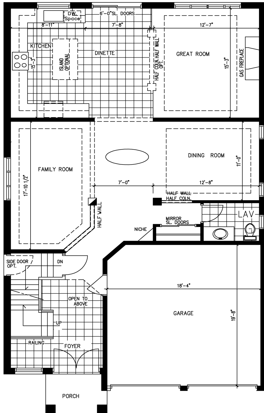
MAIN FLOOR 1282 sq.ft.
