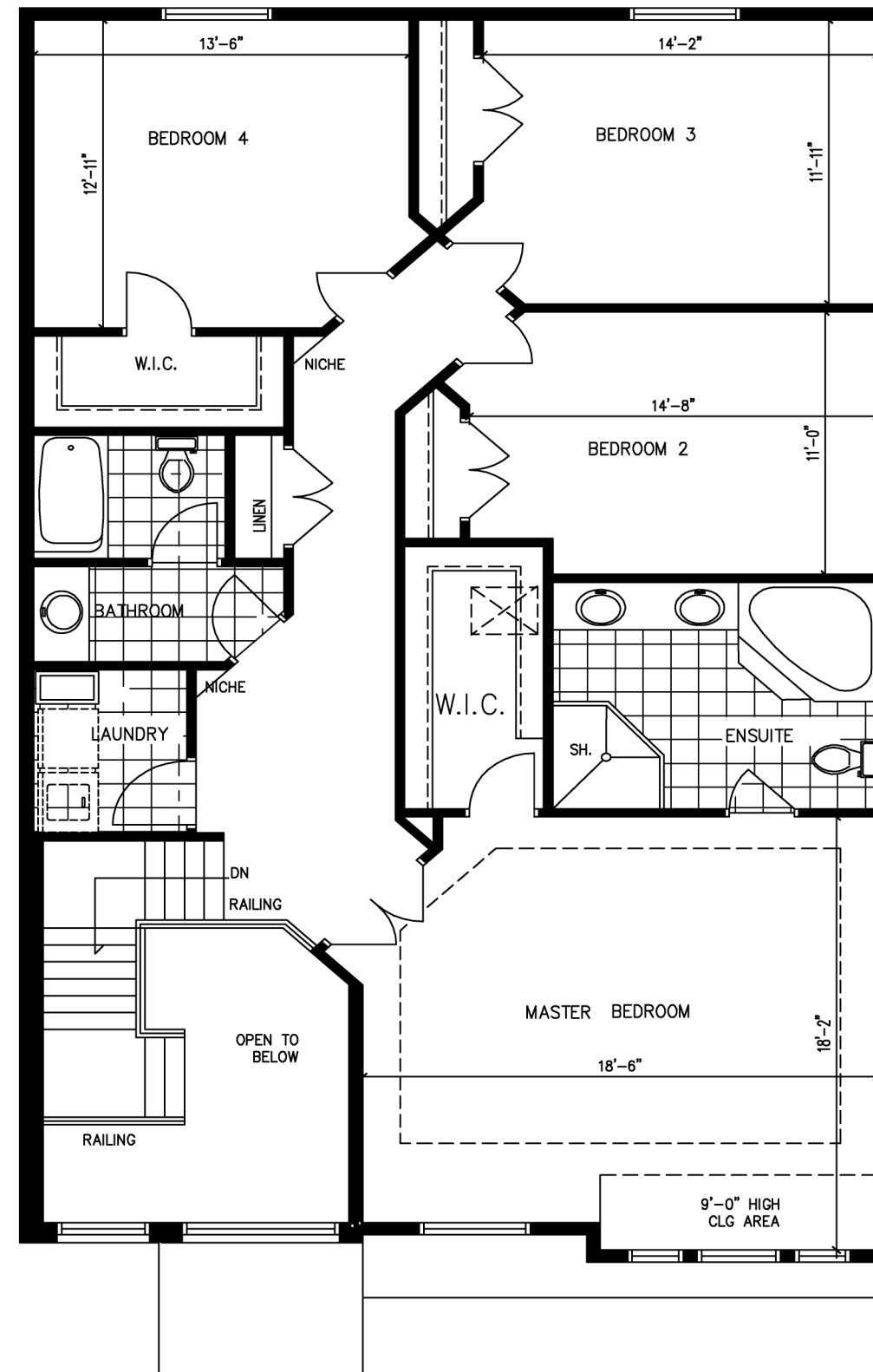
SECOND FLOOR 1629 sq.ft.
