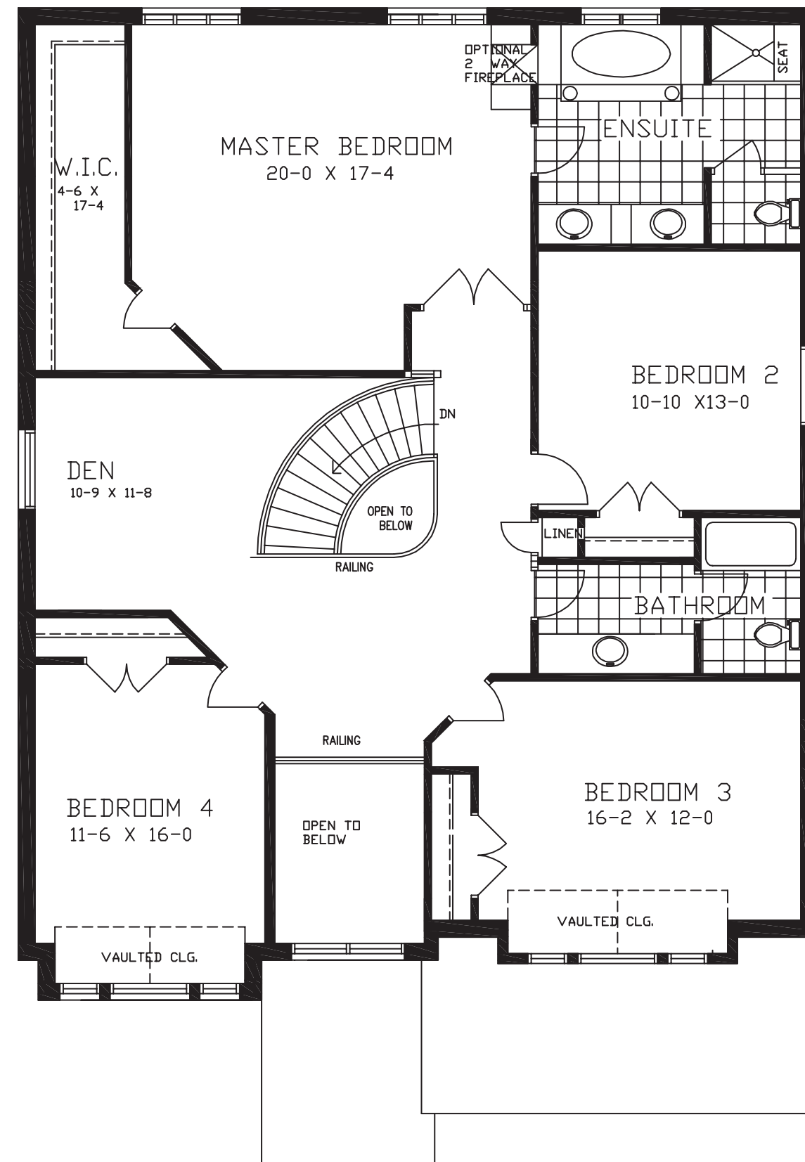
SECOND FLOOR 1920 sq.ft.
